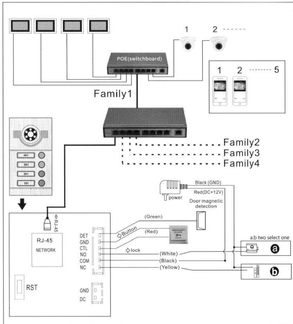
System Diagram With PoE
